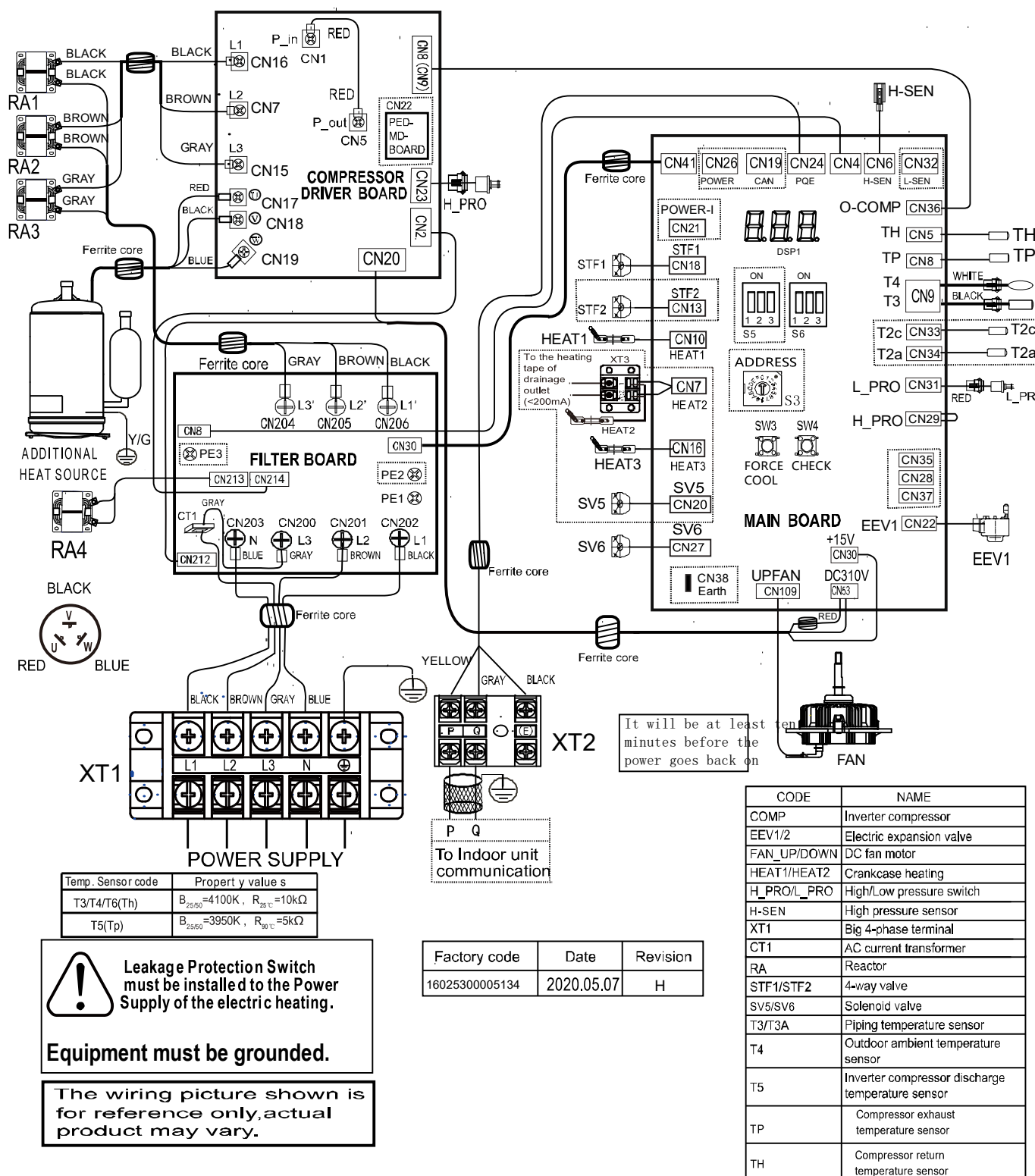
Figure 2-4.1: MSH-120EB-3; MSH-140EB-3; MSH-160EB-3 wiring diagram
