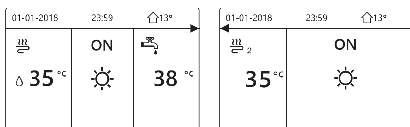
Figure 3-8.23: Set DOUBLE ZONE to YES and set ROOM TEMP. to NON; Set WATER FLOW TEMP. to YES or NON
