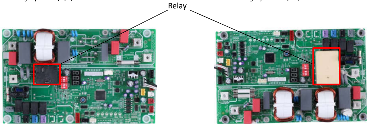
Figure 4-4.4: Relay location of main PCB for refrigerant system Single phase 4/6/8/10kW unit Single phase 12/14/16kW unit
