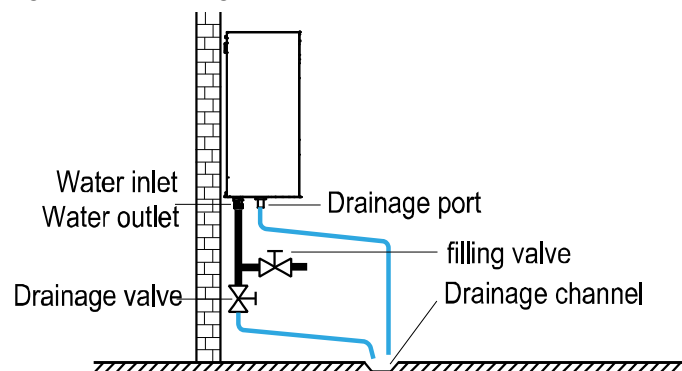
Figure 3-2.16: Drainage
