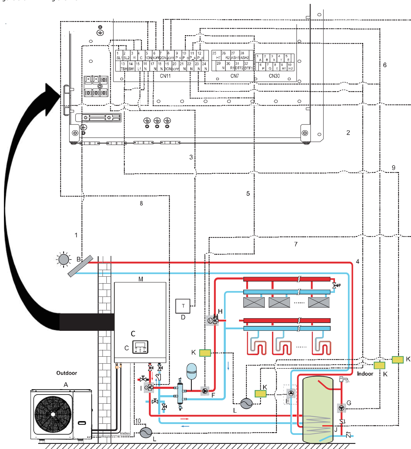
Figure 3-5.1: Wiring overview
