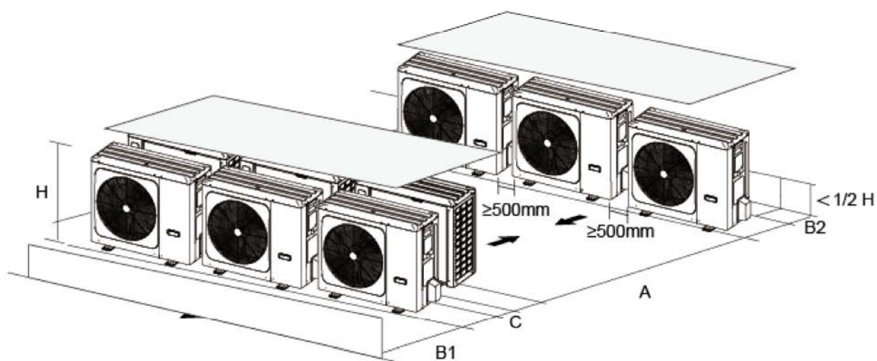
Figure 3-2.11: Multi-row installation
