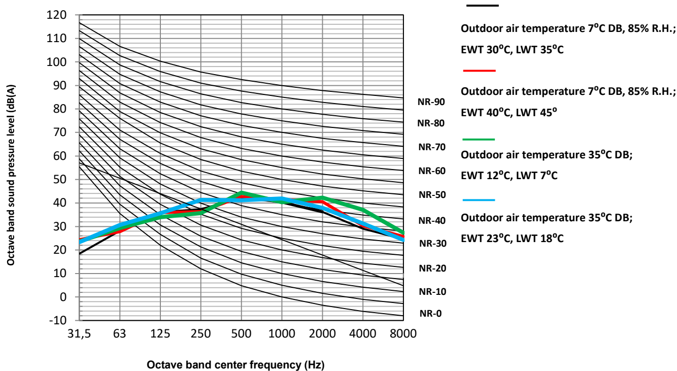
Figure 2-8.3: MSH-60EB octave band levels
