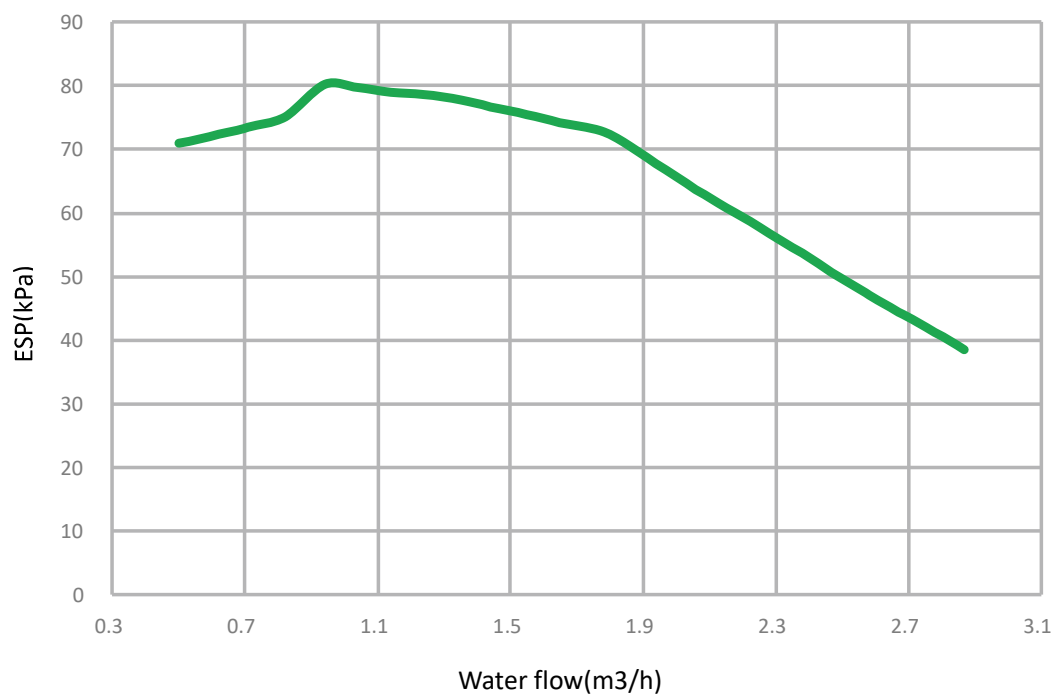
Figure 2-7.2: MSH-160IB; MSH-160IB/3; MSH-160IB-3/9 hydronic performance
