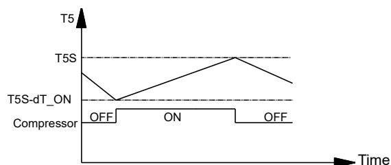
Figure 3-8.5: dT5_ON
