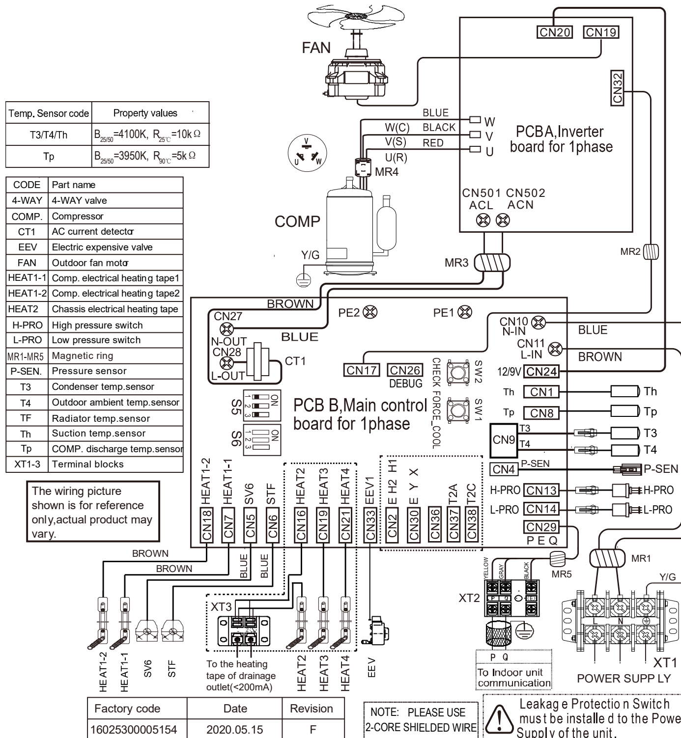
Figure 2-4.1: MSH-40EB; MSH-60EB; MSH-80EB; MSH-100EB wiring diagram
