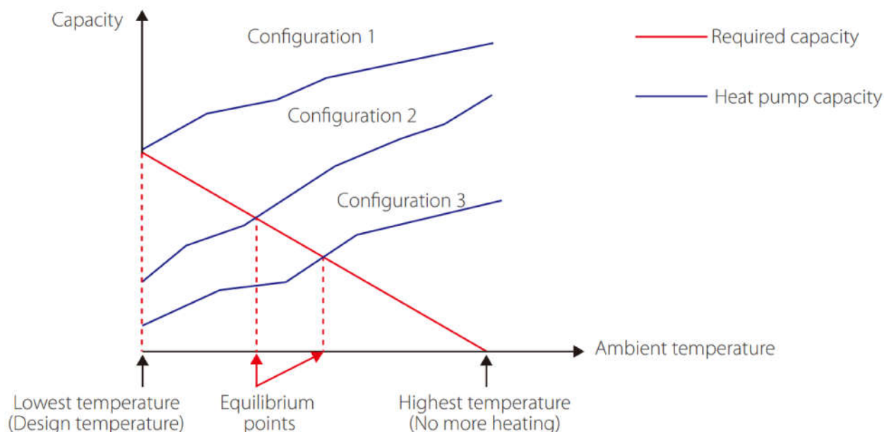
Figure 1-1.2: System configurations
