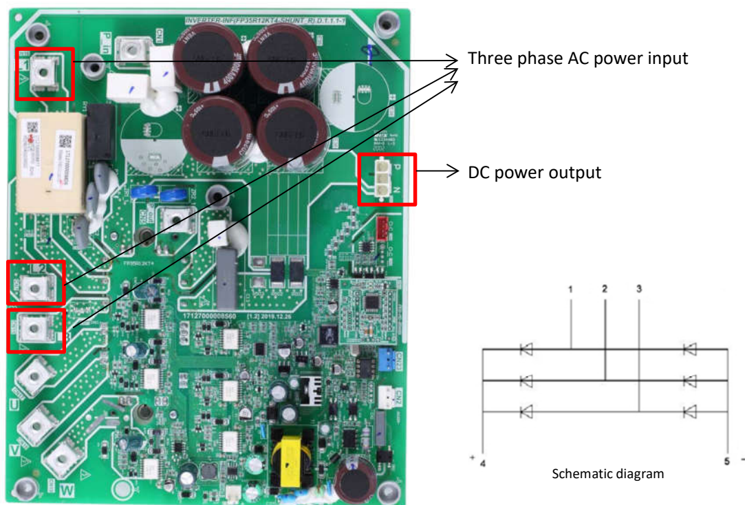
Figure 4-4.11: Bridge rectifier
