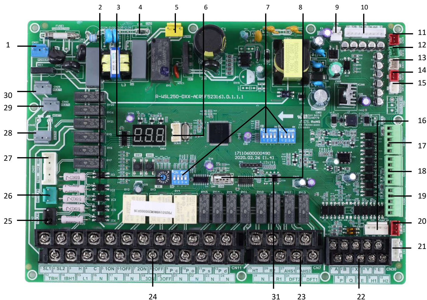
Figure 4-2.1: MSH-60IB; MSH-60IB/3; MSH-100IB; MSH-100IB/3; MSH-100IB-3/9; MSH-160IB; MSH-160IB/3; MSH-160IB-3/9
