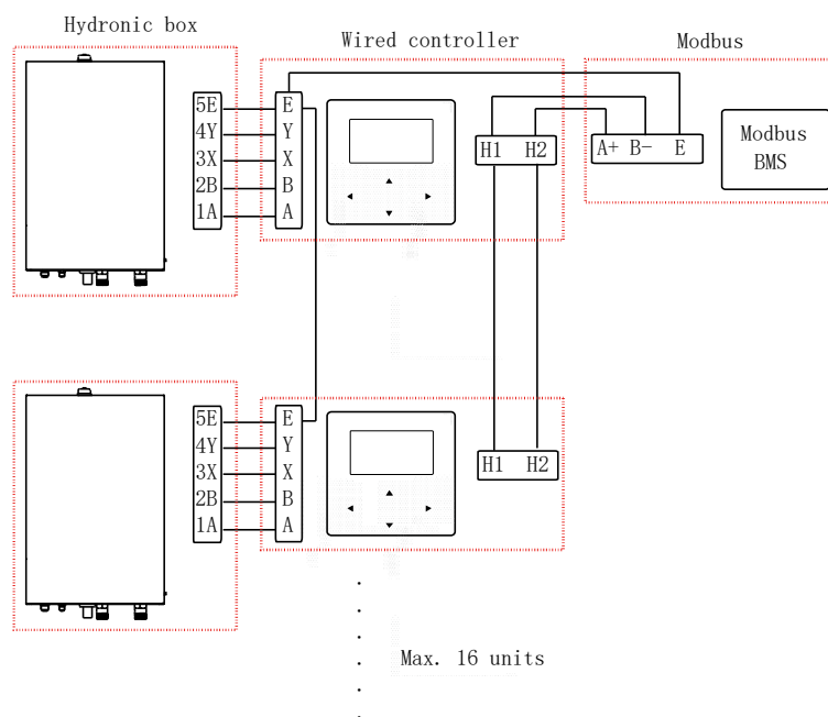
Figure 4-2.11: Connection
