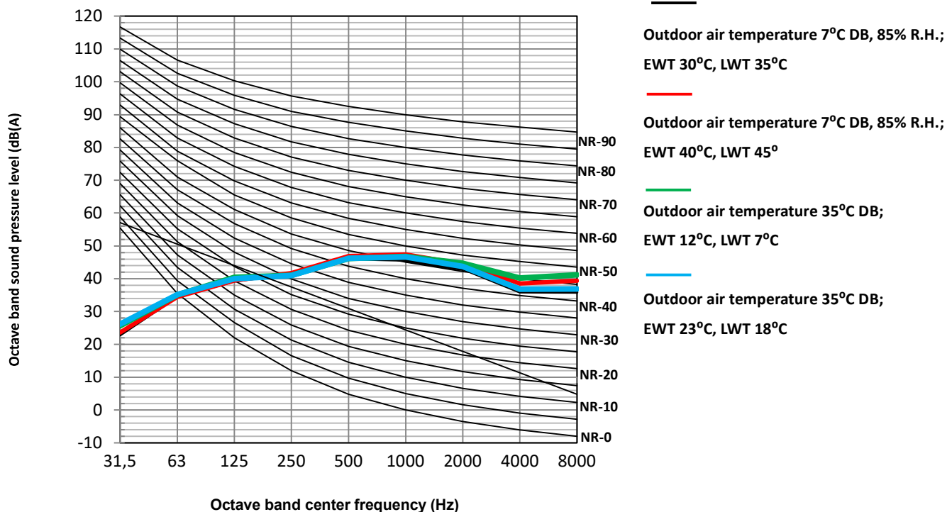
Figure 2-8.5: MSH-120EB-3 octave band levels
