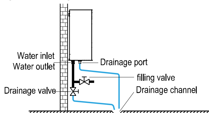
Figure 3-2.16: Drainage
