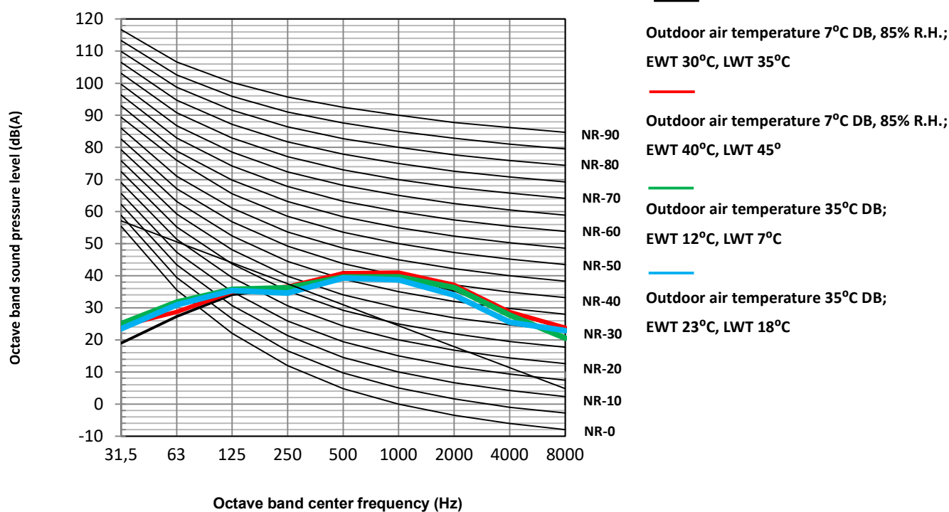
Figure 2-8.2: MSH-40EB octave band levels
