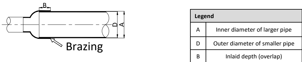
Figure 3-3.8: Piping overlap and gap for brazed joints
