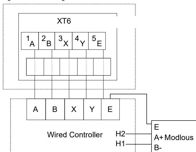
Figure 4-2.12: Wiring
