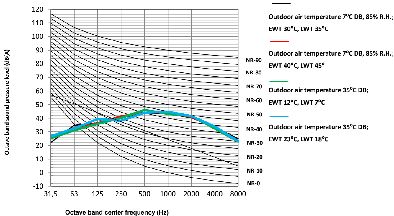
Figure 2-8.4: MSH-80EB octave band levels
