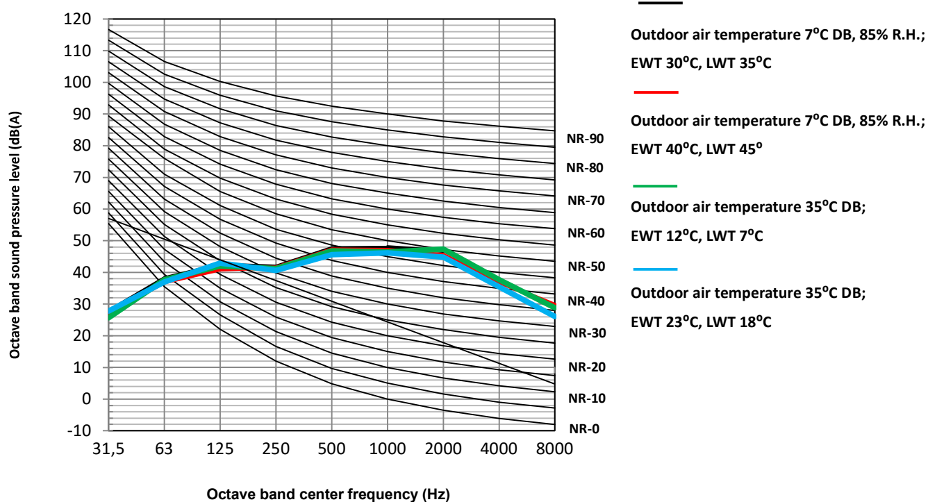
Figure 2-8.5: MSH-140EB octave band levels
