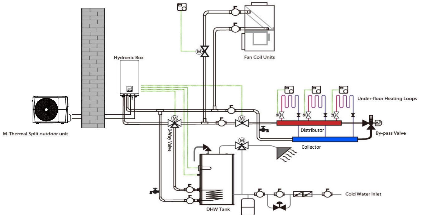
Figure 1-1.1: System schematic
