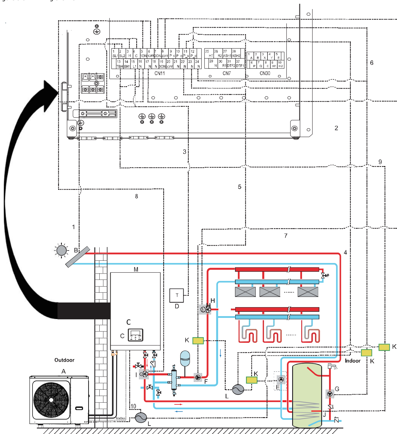
Figure 3-5.1: Wiring overview
