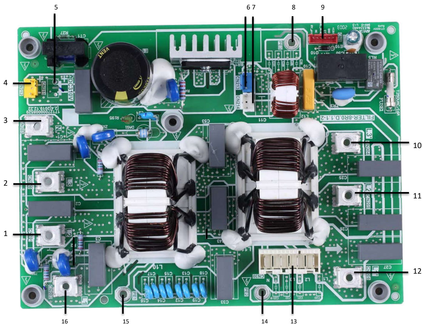
Figure 4-2.8: MSH-120EB-3; MSH-140EB-3; MSH-160EB-3 outdoor unit filter board
