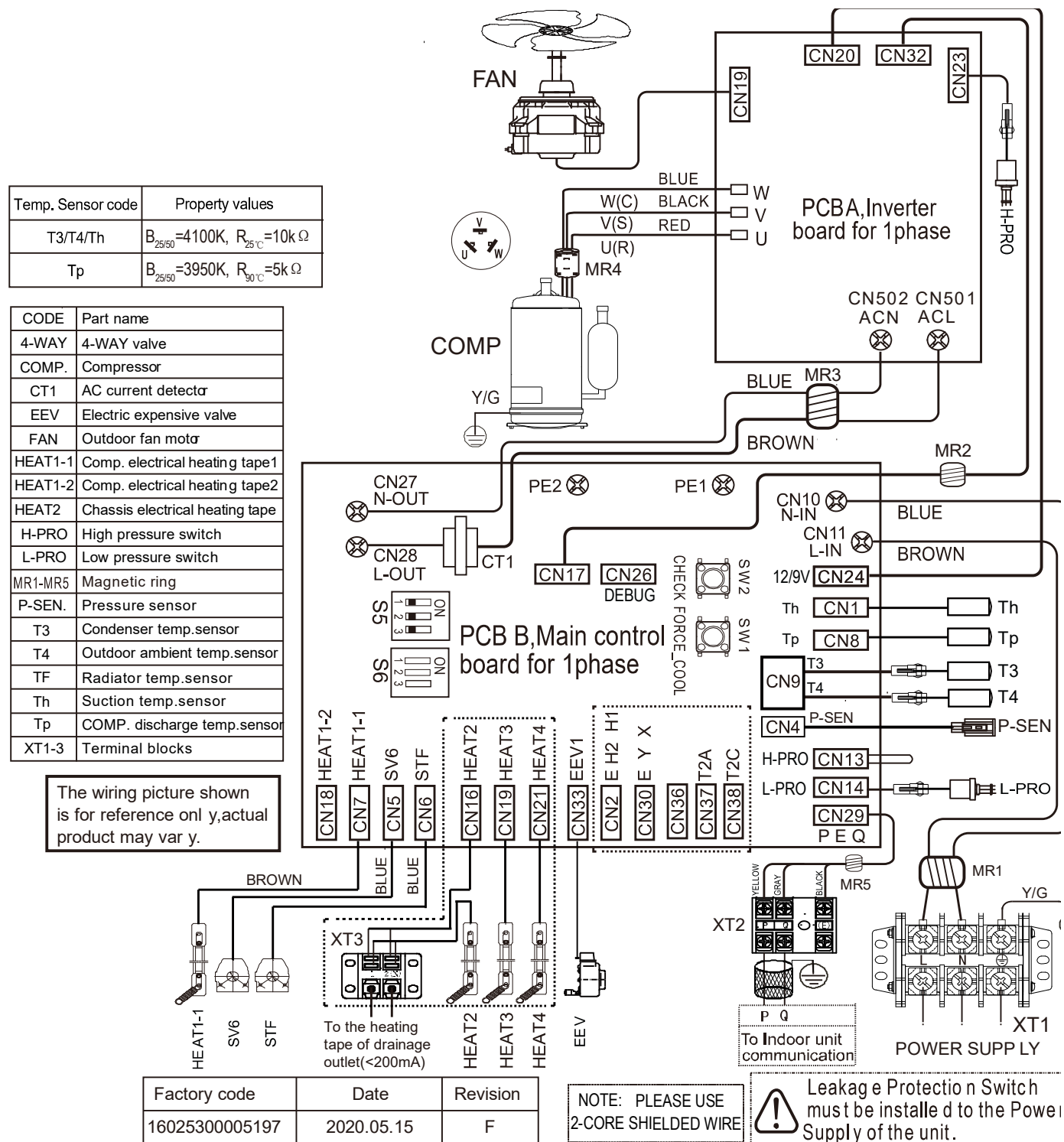
Figure 2-4.1: MSH-120EB; MSH-140EB; MSH-160EB wiring diagram
