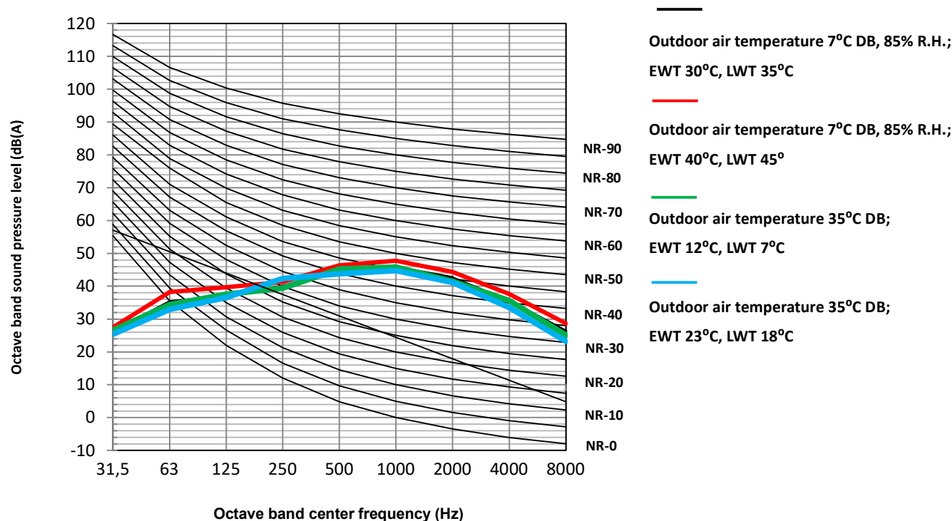
Figure 2-8.5: MSH-100EB octave band levels
