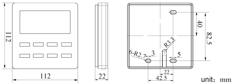
Fig. 21 Dimension of wired controller
