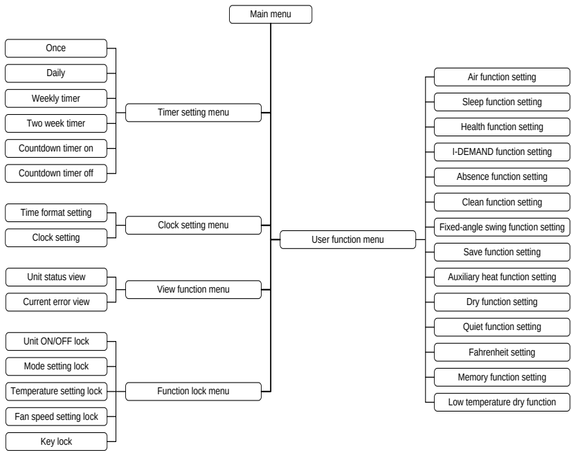
Fig. 3 Menu structure
