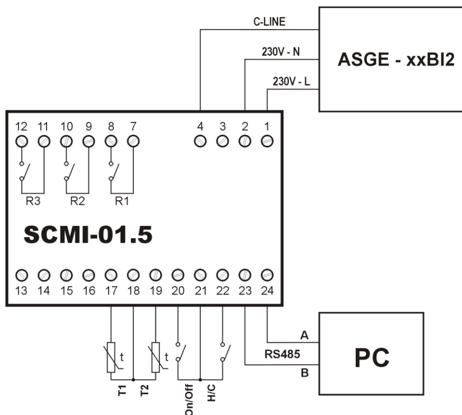
Fig. 6. SCMI-01.5 control module in the switched heating/cooling mode
