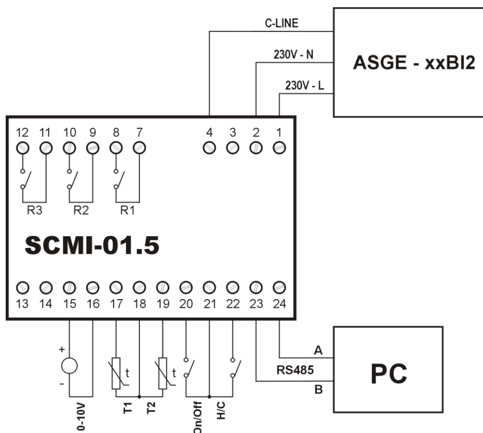
Fig. 3. SCMI-01.5 control module in the slave mode Reg.U
