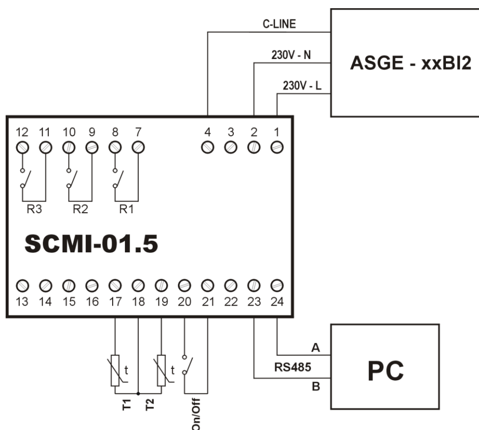
Fig. 5. SCMI-01.5 control module in the autonomous supply air temperature control mode
