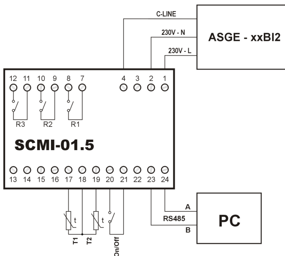
Fig. 4. SCMI-01.5 control module in the slave mode Reg.M
