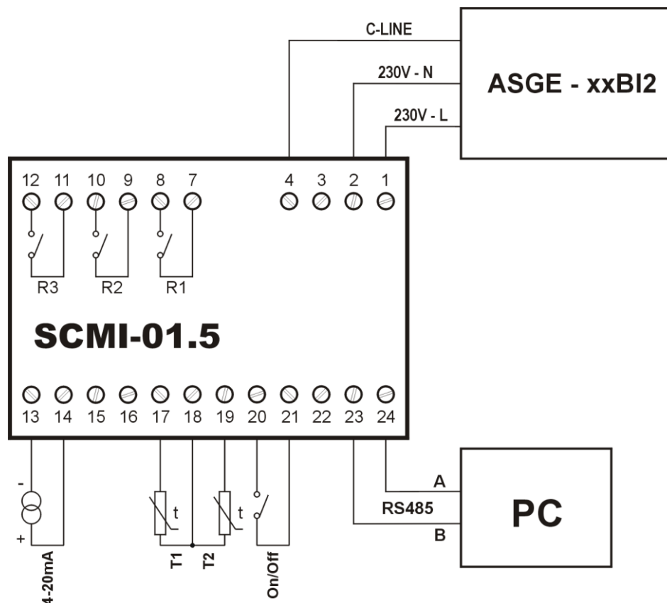
Fig. 7. SCMI-01.5 control module in the autonomous pressure control mode affected by T2 temperature
