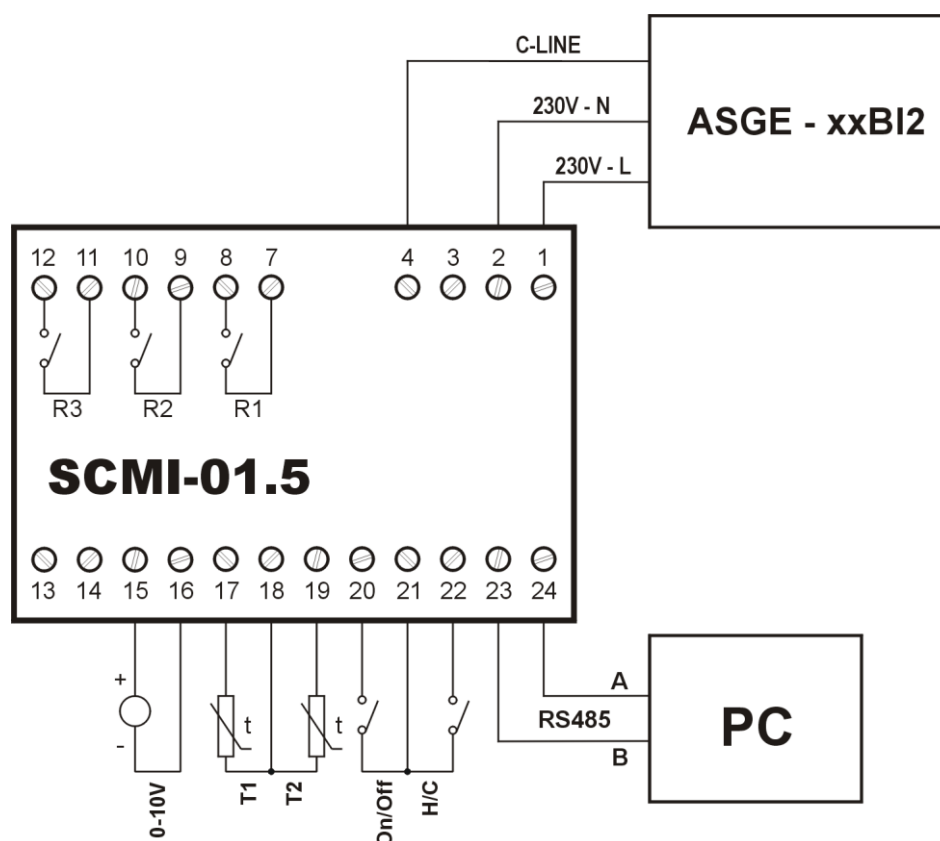
Fig. 8. SCMI-01.5 control module in the switched heating/cooling mode with temperature correction by using voltage of 0-10V
