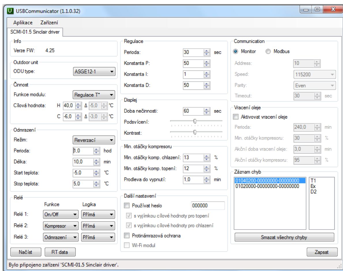
Fig. 10. Default settings of the SCMI-01.5 module
