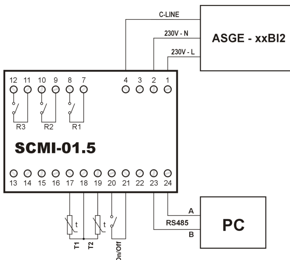
Fig. 9. SCMI-01.5 control module in the autonomous supply air temperature control mode
