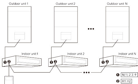
Fig. 5.5 One wired controller controls multiple UNI split 2 units simultaneously
