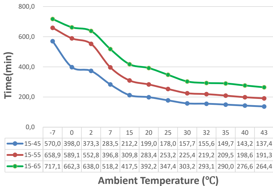
Heat Up Time within Different Temperature
