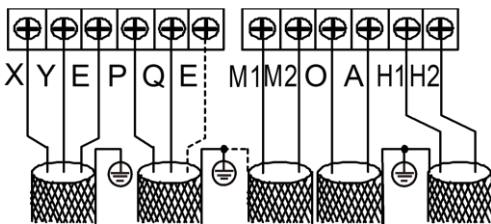
Figure 3-9.11: Outdoor unit communication terminals
