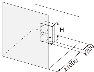
Figure 2-3.9: One outdoor unit installation (unit: mm)
