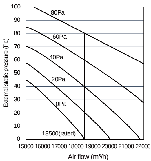
Figure 3-3.6: 16HP units fan performance
