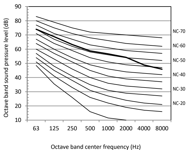
Figure 2-10.6: 16HP octave band level
