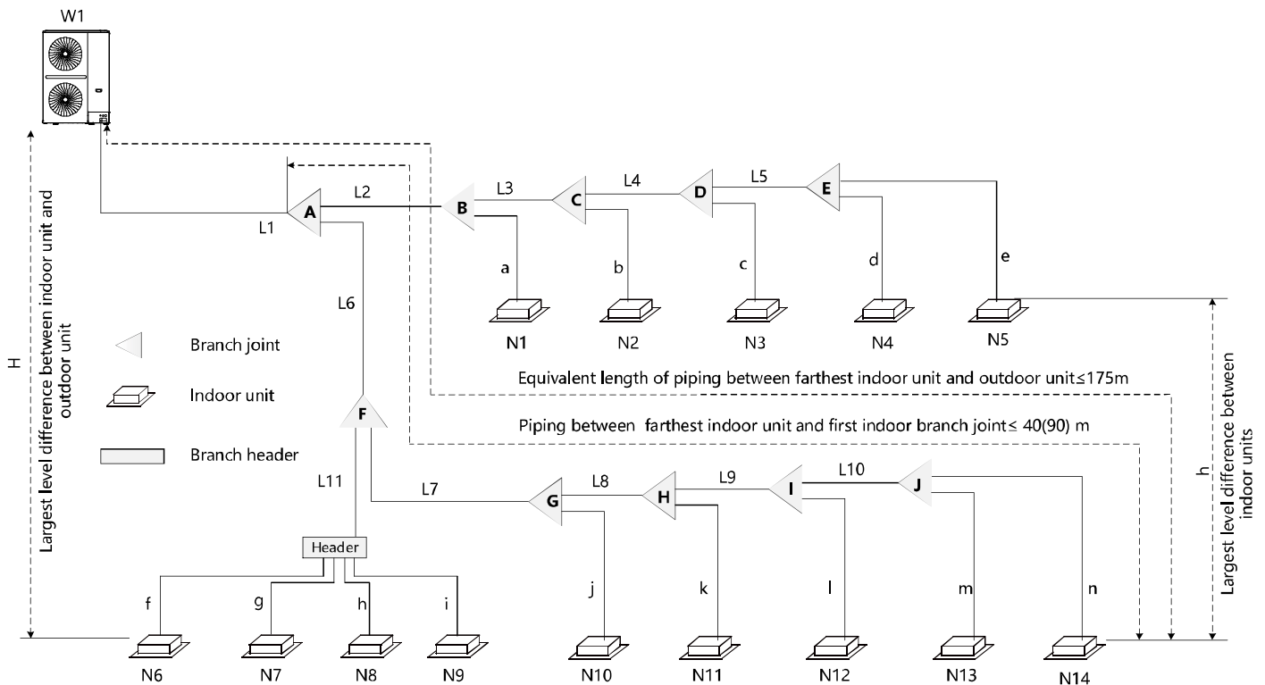
Figure 3-4.3: Selecting piping diameters
