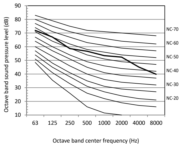
Figure 2-10.5: 14HP octave band level
