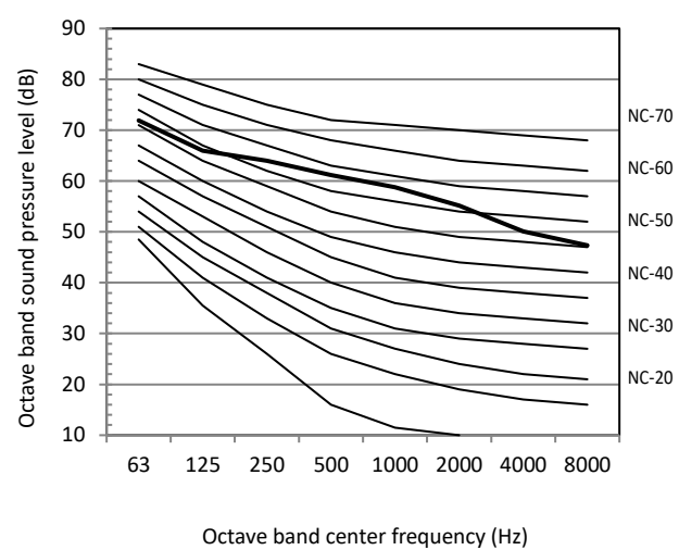
Figure 2-10.9: 22HP octave band level
