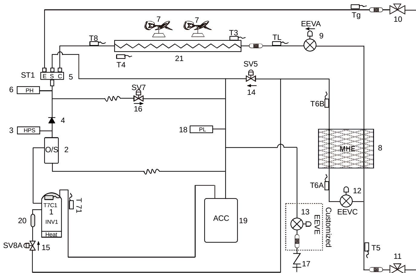
Figure 2-4.1: 8-14HP piping diagram
