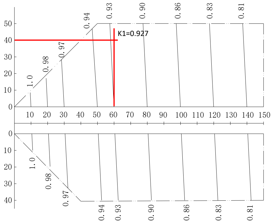
Figure 1-6.3: SDV6 rate of change in cooling capacity
