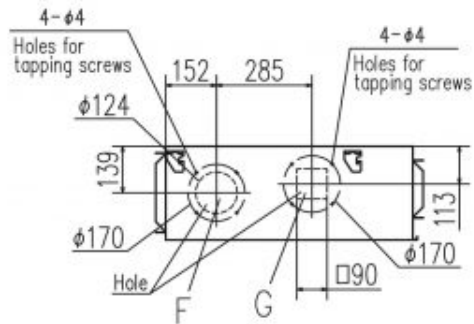
View M
