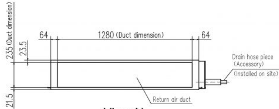
View N
