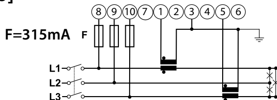
[6] 3 phases, 3 wires, unbalanced load
