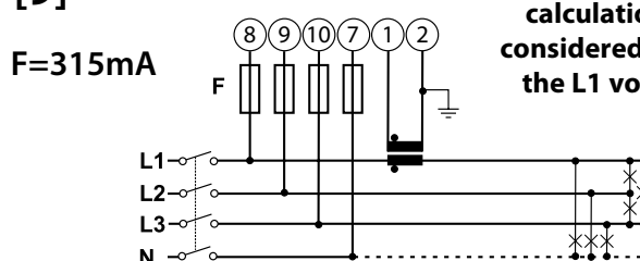
[9] 3 phases, 3/4 wires, balanced load
