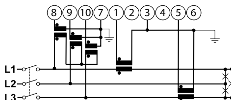
[7] 3 phases, 3 wires, unbalanced load
