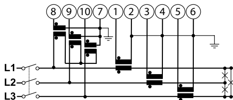
[4] 3 phases, 3 wires, unbalanced load
