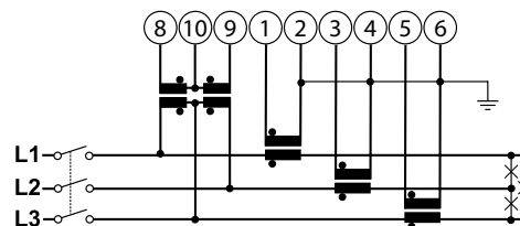
[5] 3 phases, 3 wires, unbalanced load
