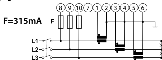
[3] 3 phases, 3 wires, unbalanced load
