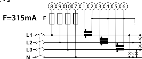
[1] 3 phases, 4 wires, unbalanced load
