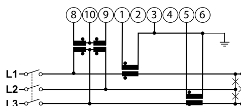
[8] 3 phases, 4 wires, unbalanced load
