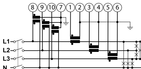
[2] 3 phases, 4 wires, unbalanced load
